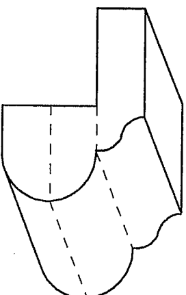
2 1/4" OGEE BULLNOSE
