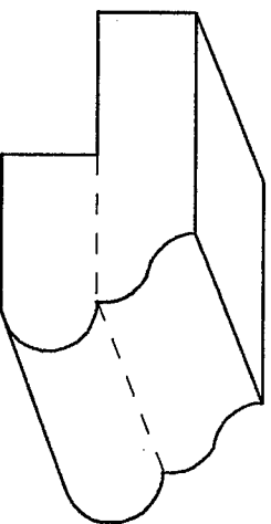
1 1/2" OGEE BULLNOSE
